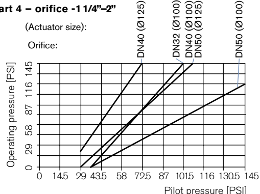
Chart 4 - orifice 1 1/4"-2"
