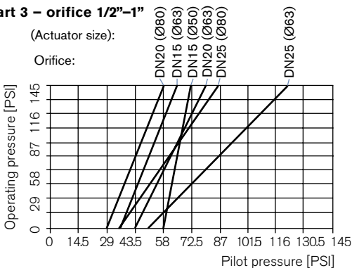
Chart 3 - orifice 1/2"-1"
