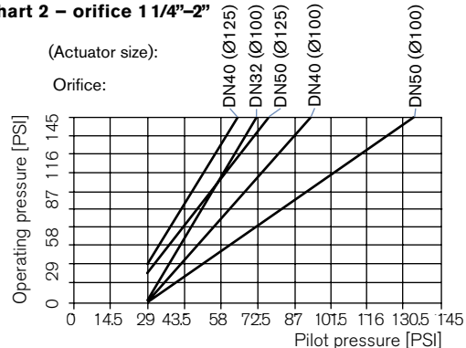
Chart 2 - orifice 1 1/4"-2"
