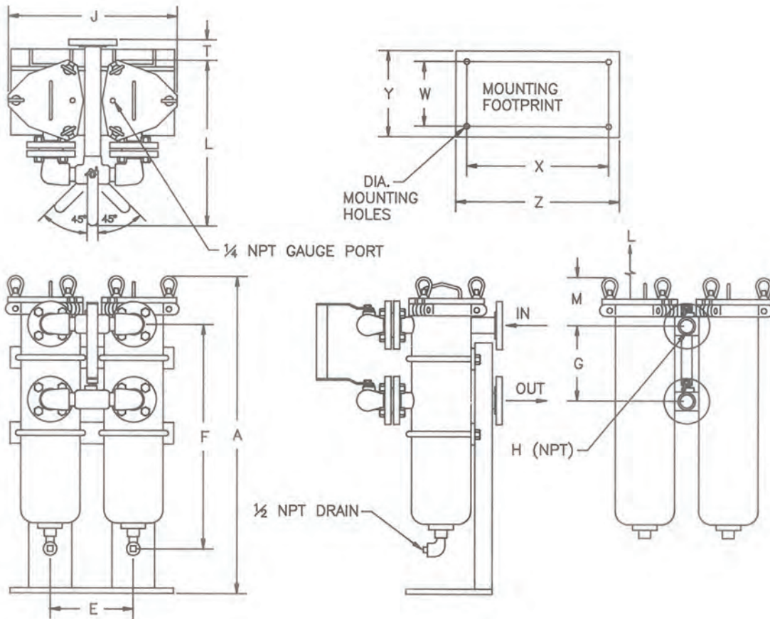
DUPLEX ASSEMBLY DIMENSION TABLE
